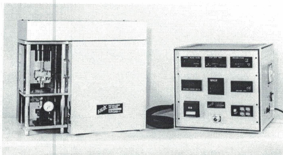
FIG. 1 The Falex Multispecimen Test Machine
