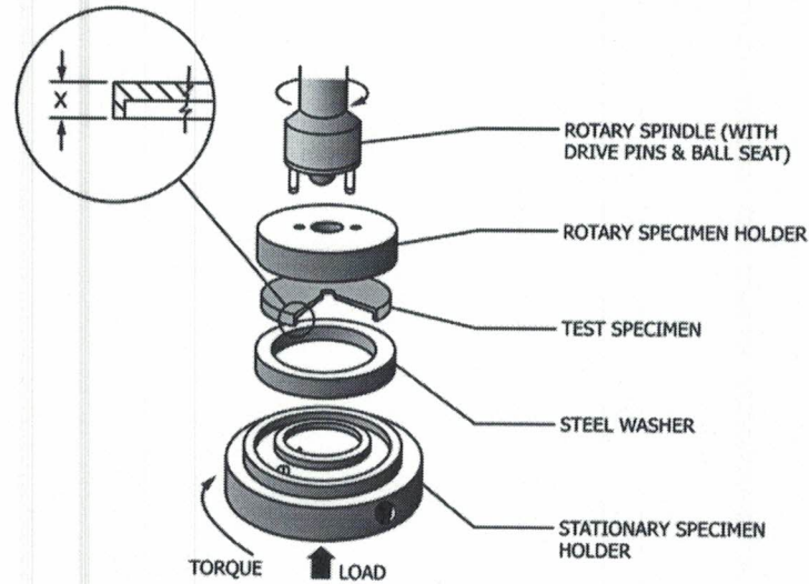
FIG. 2 Thrust Washer Test Specimen Arrangement
