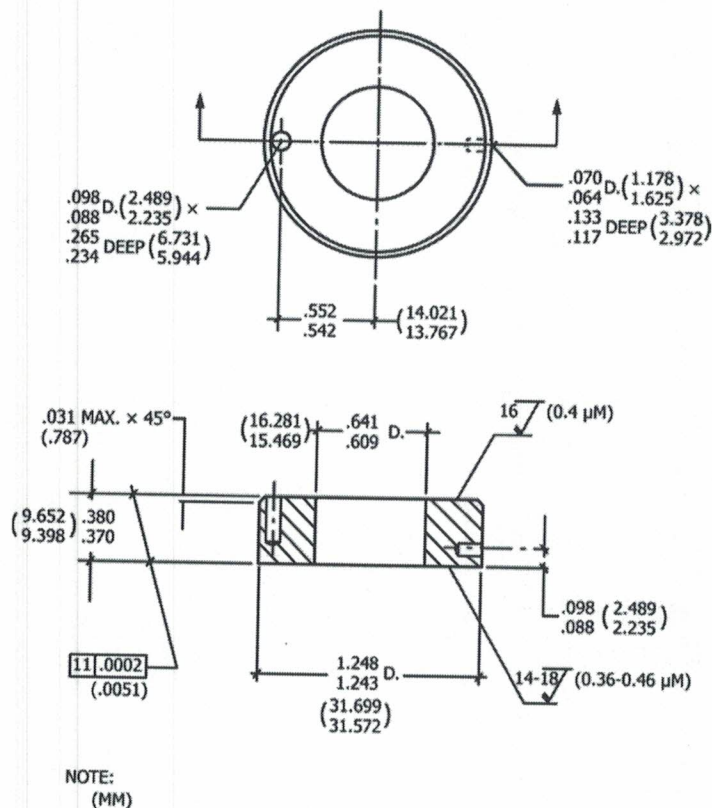
FIG. 4 Stationary Steel Washer Specimen
