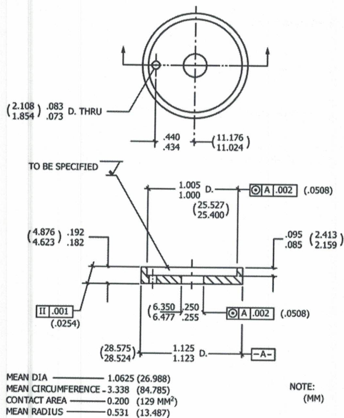
FIG. 3 Rotating Test Specimen
